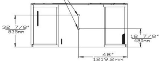
VIEW "B"
